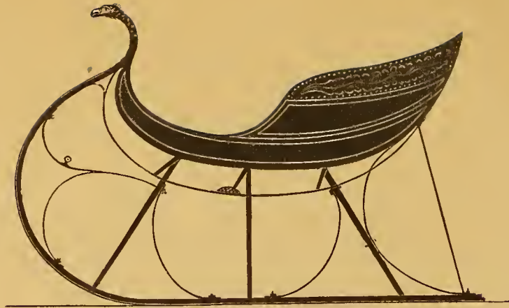
CUTTER SLEIGH.— \frac{1}{2} IN. SCALE.
